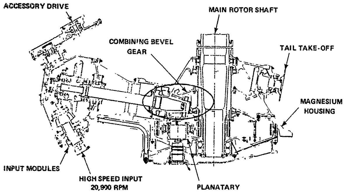
Figure 9. BLACK HAWK Main Gearbox
