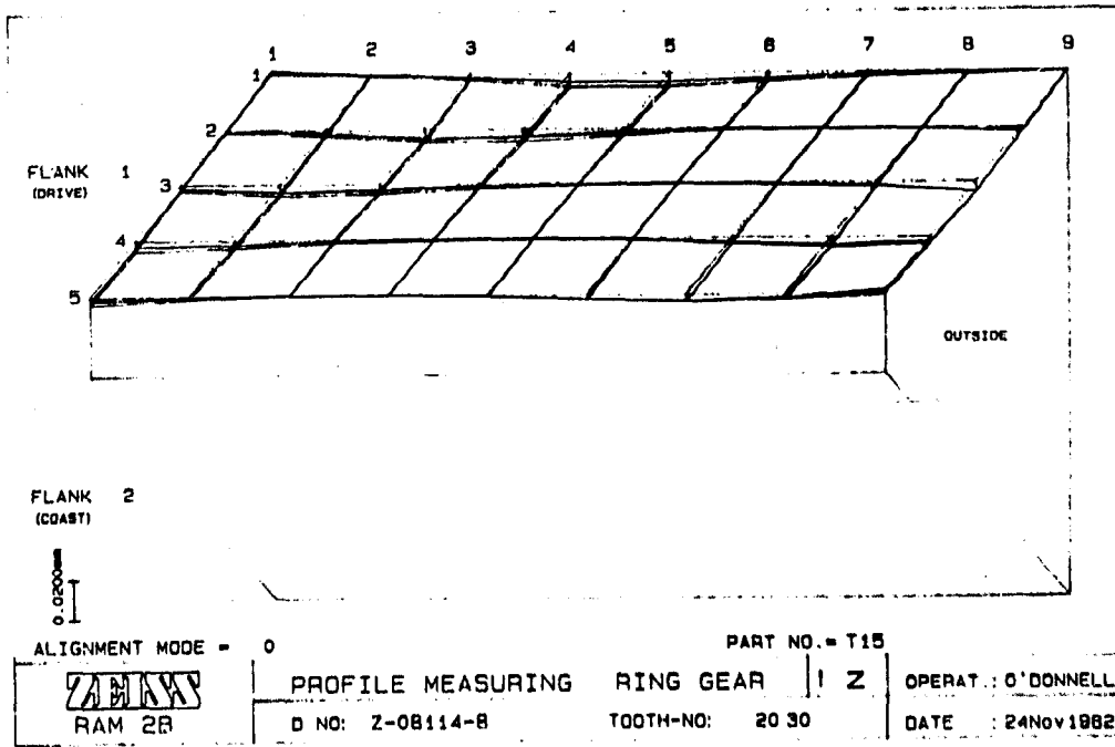
Figure 20. Zeiss Measurements of Master Gear
