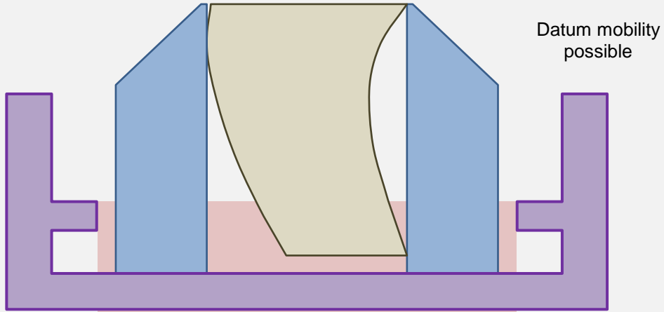
Untilted cylinder at Minimum-Material (UAME)
