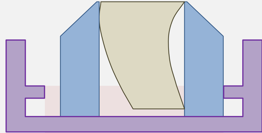
Untilted cylinder at Minimum-Material (UAME)
